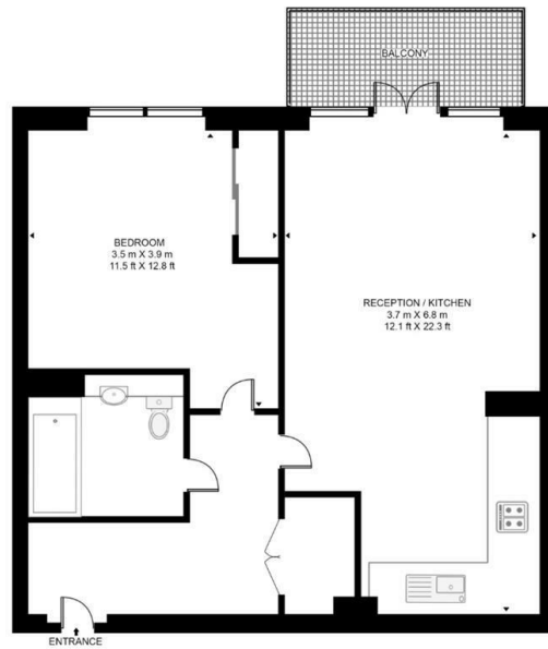
FOURTH FLOOR
